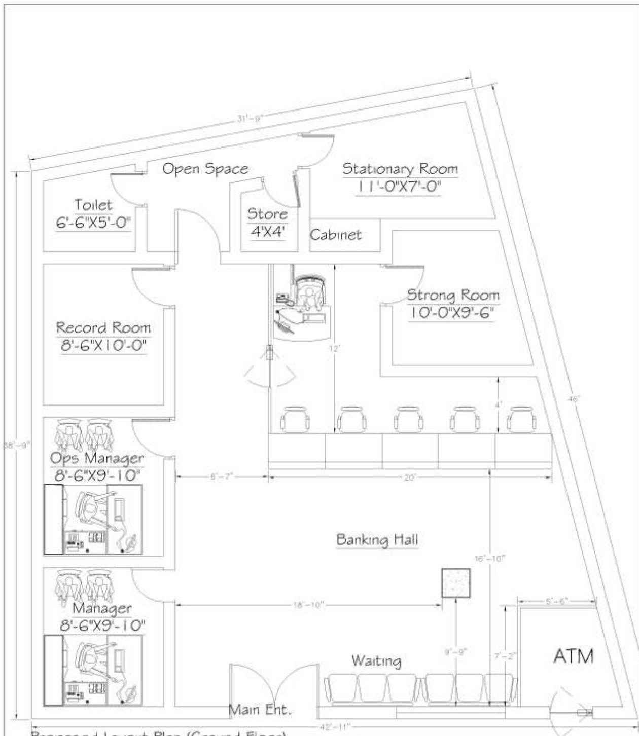
Proposed Layout Plan (Ground Floor) Branch Code # 0087 Name: P.N. Dockyard Branch Karachi South Region
