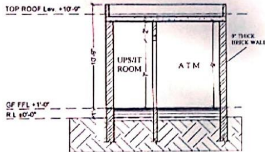
ATM & IT Room X-Section
