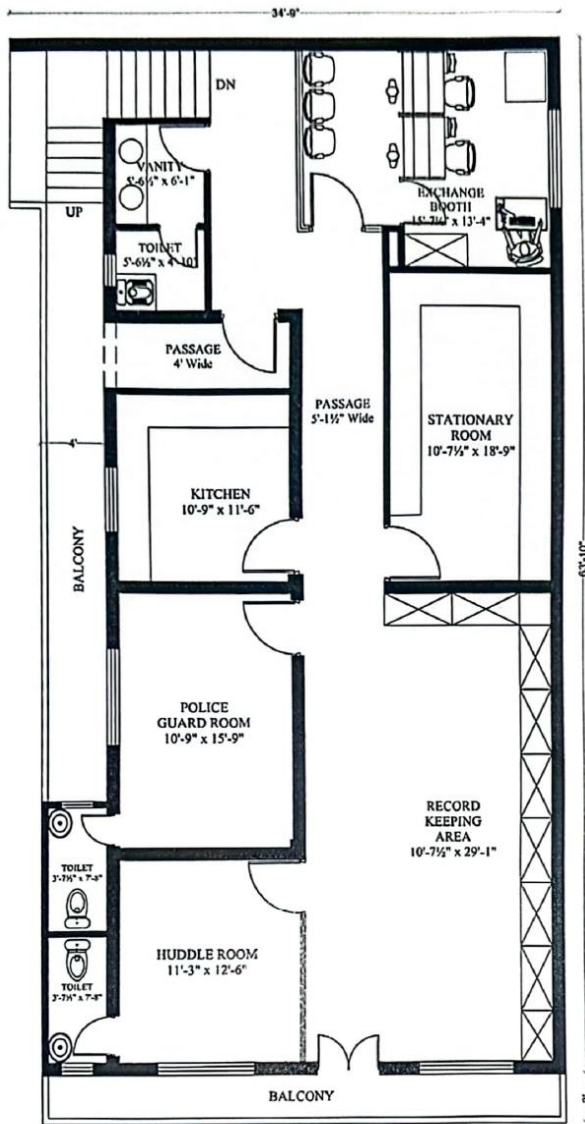
FIRST FLOOR (Proposed) 2168 SQ.FT
