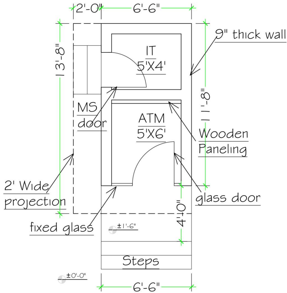
Proposed Layout Plan Army ATM Room
